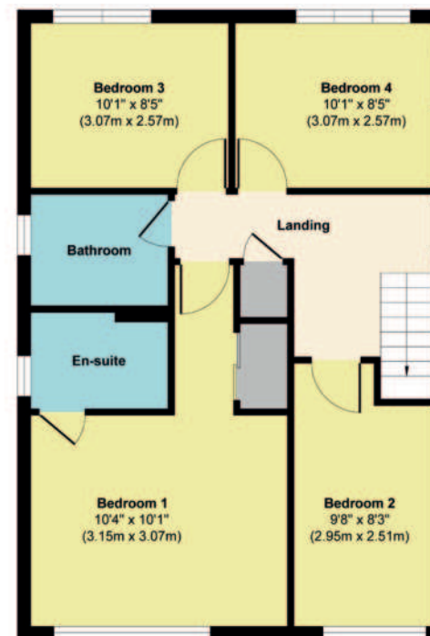
First Floor Approximate Floor Area 630 sq. ft (58.52 sq. m)
